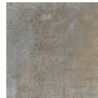
Fusion Oxide
